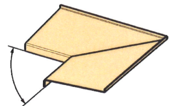
Inneneck-Dilatation
